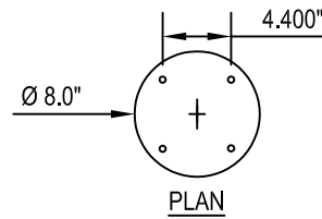
STEEL INSERT TO FIT THRU BOTTOM
