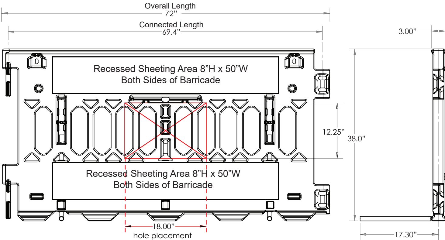
Sign Area: Holds 20"W x 14"H Sign on each side (screw on)
